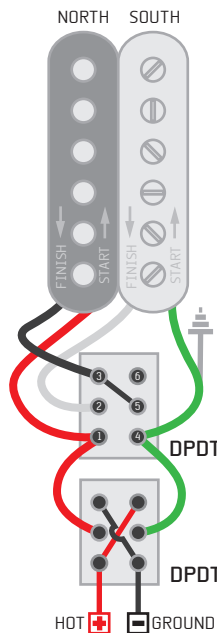
DUAL SOUND & PHASE SWITCH (Switch between Serial & Parallel sounds)
