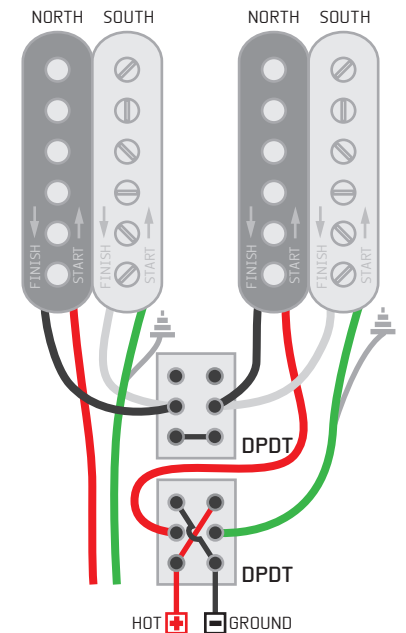
SINGEL COIL & PHASE SWITCH (Switch between Humbucking & single Coil + phase switch)
