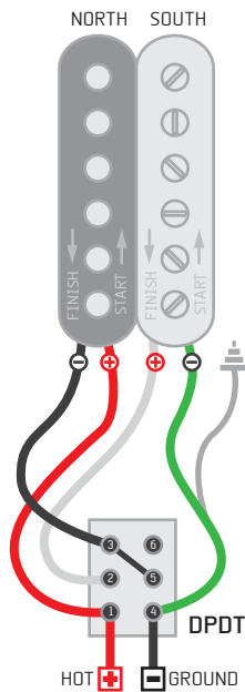
DUAL SOUND (Switch between Serial & Parallel sounds)
