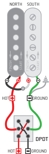
PICKUPS OUT OF PHASE (Only need ONE switch on ONE pickup)
