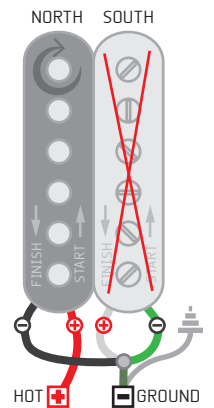
COIL CUT (Ground out, 1 coil, No humbucking) F+F+S+BRAID=GROUND LEAD S=HOT LEAD
