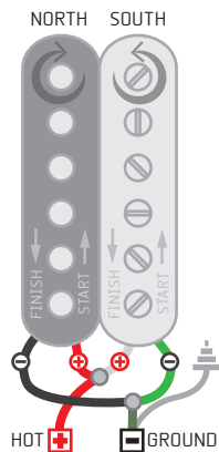
PARARELL/OUT OF PHASE (Humbucking w/single coil sound) F+S+BRAID=GROUND LEAD F+S=HOT LEAD
