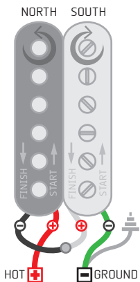
SERIES/OUT OF PHASE (Most common) F+F=SERIES LINKED S+BRAID=GROUND LEAD S=HOT LEAD
