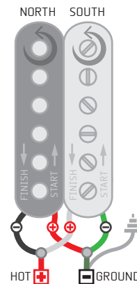
PARARELL/IN PHASE (No humbucking) S+S+BRAID=GROUND LEAD F+F=HOT LEAD
