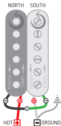
SERIES/IN PHASE (No humbucking) F+S=SERIES LINKED F+BRAID=GROUND LEAD S=HOT LEAD
