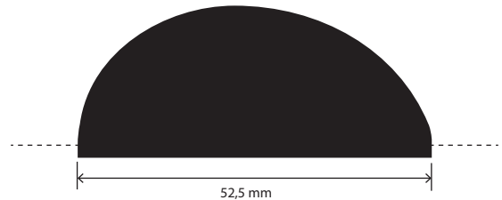
Progressive asymmetric neck shape (3 mm) Fret 13
