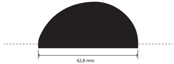
Progressive asymmetric neck shape (3 mm) Fret 1
