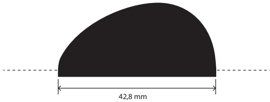
Progressive asymmetric neck shape (5 mm) Fret 1
